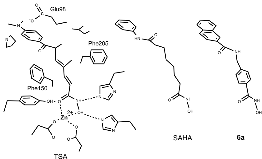
Figure 1. Proposed molecular shapes of TSA, SAHA and 6a packing in the HDAC pocket, which were prepared by modifying the TSA-HDL (histone deacetylase like protein) binding representation in Figure 3 illustrated in Ref. 6.
